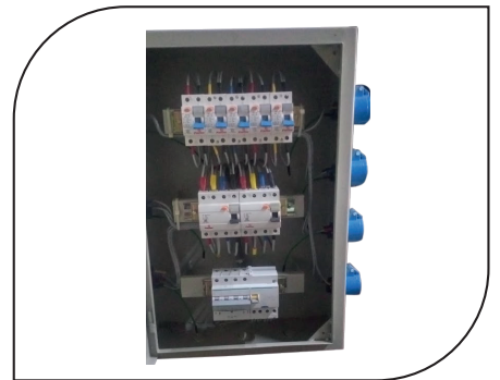
PANEL BOX
