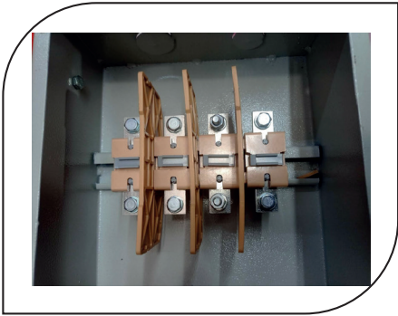
CONNECTOR BOX
